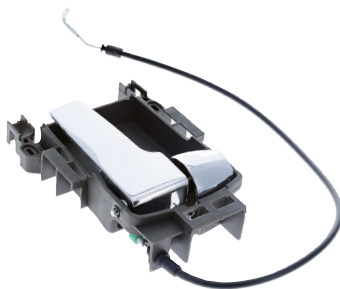
775-5217 Kenworth 2020-05 (Front Right, Gray Housing w/Chrome Lever; w/cable) OE Numbers: R251100228111RSC, R561063R
